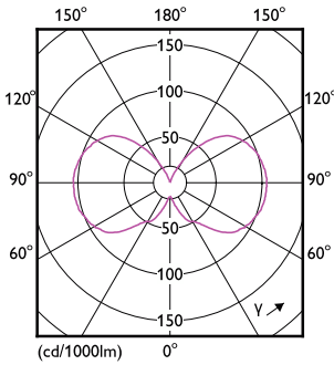
Light Distribution Diagram - LEDClassic 4.5W A15 E27 850 CL ND 1PF/10
