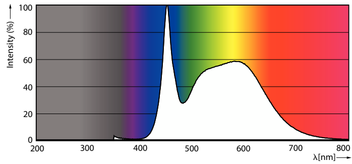
Spectral Power Distribution Colour - LEDClassic 4.5W A15 E27 850 CL ND 1PF/10
