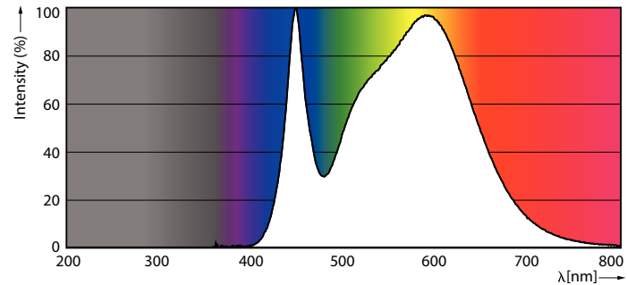
Spectral Power Distribution Colour - TForce Core HB 30W E27 840 CN GN3
