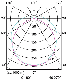
Light Distribution Diagram - 60WP/LED/840/ND EX39 G2 BB 6/1
